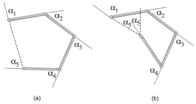
Figure 6: Simple pruning test for self collision detection based on angles: if \sum_{i=0}^{i<n} \|\alpha_i\| <= 2\pi , then self-intersection can not occur.
